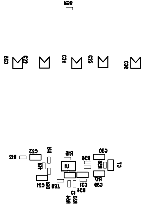
Figure 46. PCB Bottom-Side Silkscreen
